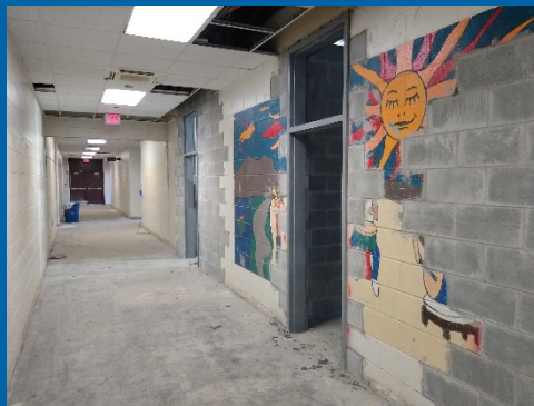
Installation of Door Frames in Masonry Walls
